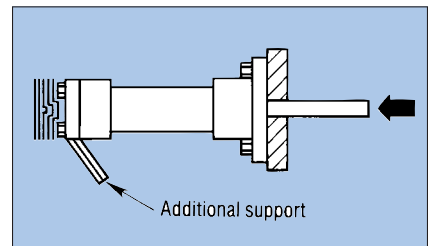
Fig. 17. An overhung cylinder needs additional support to prevent cylinder movement at non-flange end. Cylinder length changes with pressure and temperature.
