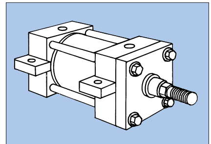
FIG. 12. As with other NFPA standardized mountings, centerline lug mounts provide straight-line transfer of force.
