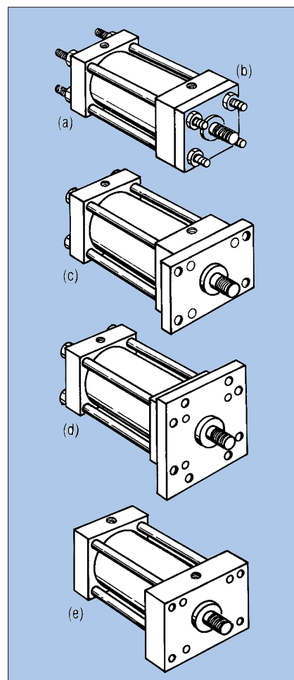
Fig. 11. Fixed cylinder mounts that provide straight-line force transfer are: (a) tie rods extended, and extended both ends (a + b); (c) head rectangular flange, (d) head square flange; and (e) rectangular head which provides same service as (c) but uses entire head rather than an added flange. Cap flange mounts are the same as (c) and (d) but bolt to cap (not shown). Rectangular caps also are available.
