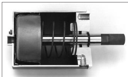
Fig. 10. By eliminating the conventional sliding piston seal — and its inherent tendency toward stick-slip operation — diaphragm cylinders produce nearly frictionless motion, except for the miniscule amount of friction at the rod seal. The diaphragm's positive sealing also eliminates the potential for leakage around the piston.
