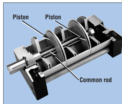
Fig. 8. Tandem cylinders use multiple pistons connected through a common rod to generate relatively high force from a low supply pressure and small bore.
