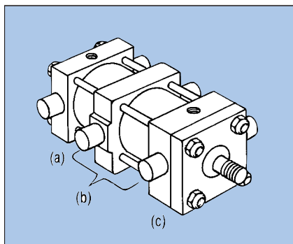
Fig. 14. Pivot mounts absorb force along centerline and actuate loads that travel through arc. Cap trunnion (a), intermediate fixed trunnion (b) can locate anywhere between head and cap, and head trunnion (c) are versions of this style; only one of these versions is used at one time. The cylinders shown in Figures 3 and 6 employ clevis mounting, which is a type of pivot mounting for loads that travel through arc.
