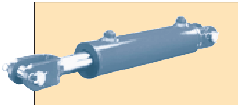
Fig. 3. Welded cylinders combine benefits of heavy-duty construction with compact design, which is the main reason why they are widely used in mobile-equipment applications.
