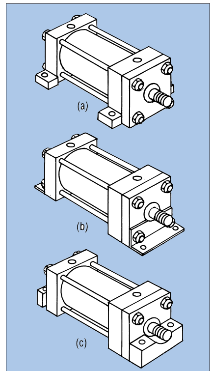
Fig. 13. Side mounted cylinders include side lug (a), side end angle (b), side and lug (c), and side tapped (not shown). These mounts produce a turning moment as the cylinder applies force to the load.
