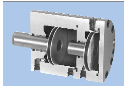
Fig. 9. Duplex cylinders have multiple pistons that are not connected to a common rod. Actuating individual piston chambers achieves multiple strokes.
