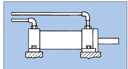
Fig. 16. Rigid tubing connected to cylinder heads will be subject to forces and motion. Cylinders plumbed this way will leak.
