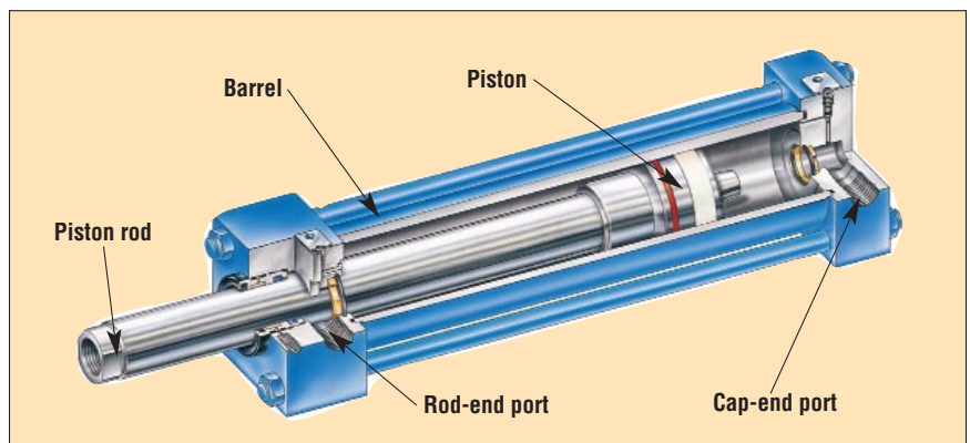
Fig. 1. Cut-away view shows key features of a typical cylinder, in this case, a double-acting model for hydraulic service with standard tie-rod construction.
