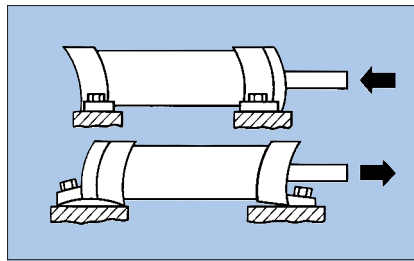
Fig. 15. Cylinders with non-centerline mountings tend to sway under load.
