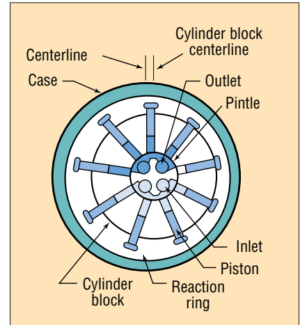
Fig. 9. Radial-piston pump.
