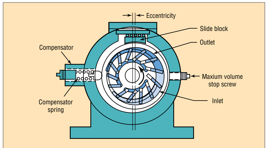
Fig. 7. Variable displacement, pressure compensated vane pump.
