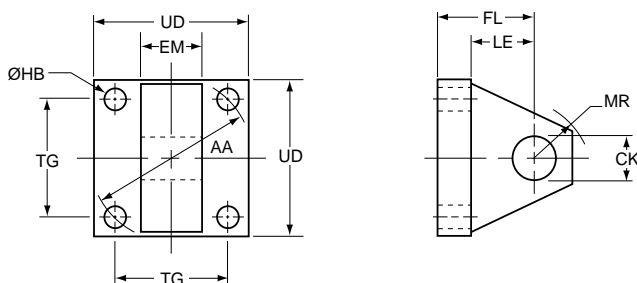
Eye Bracket
